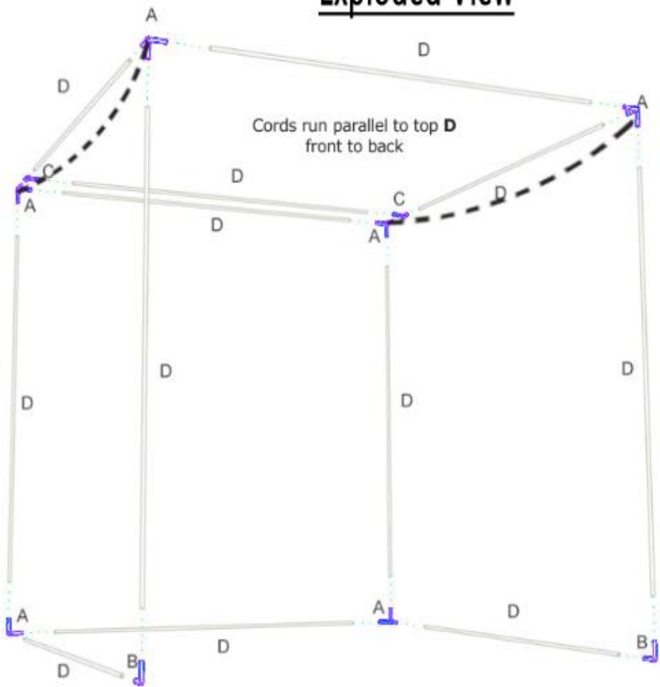
Exploded View
