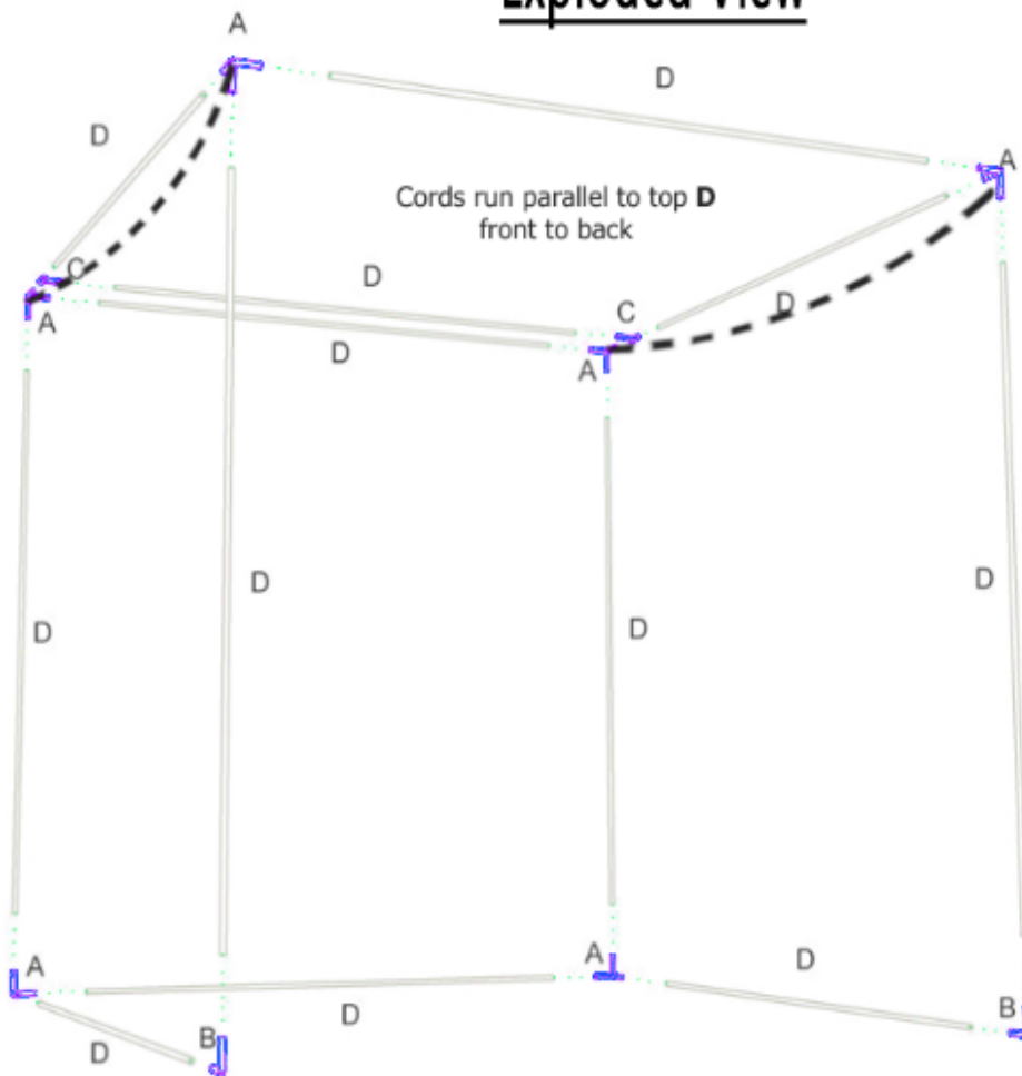
Exploded View
